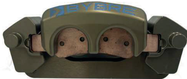
REAR CALIPER J364003M00 3P036
